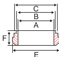
Fig. S7714PRF4 - Short Plain Bevel Seat Ferrule
