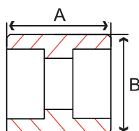
Fig. S5034CP & S5036CP - Full Coupling
