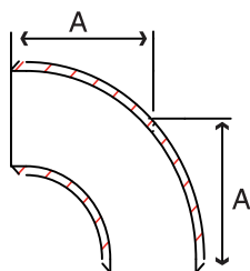
Fig. S2044LE & S2046LE - 90° Elbow Long Radius
