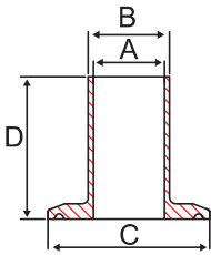
Fig. S7714MPHT6 - Tygon® Hose Adapter
