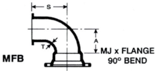
CODOS 90°: MJ x BRIDA
