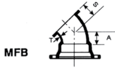
CODOS 45°: MJ x BRIDA
